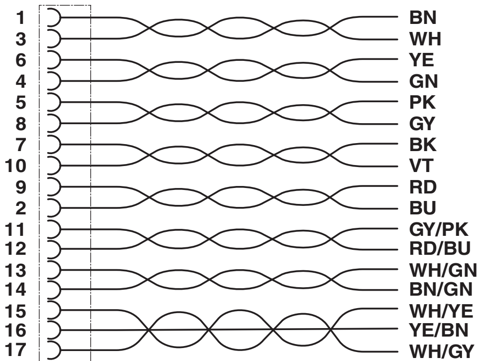
Circuit diagram
