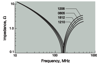
Variation of Impedance with Chip Size Impedance vs. Frequency 1000 pF - COG (NP0)
