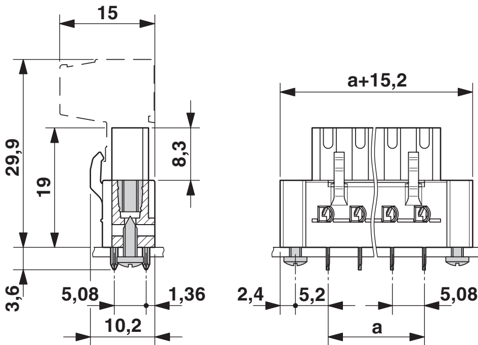
Dimensional drawing
