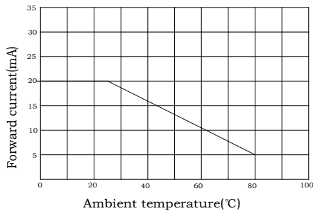
Current and ambient temperature
