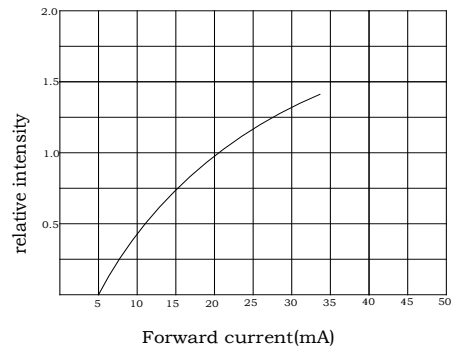
Relative light intensity vs current
