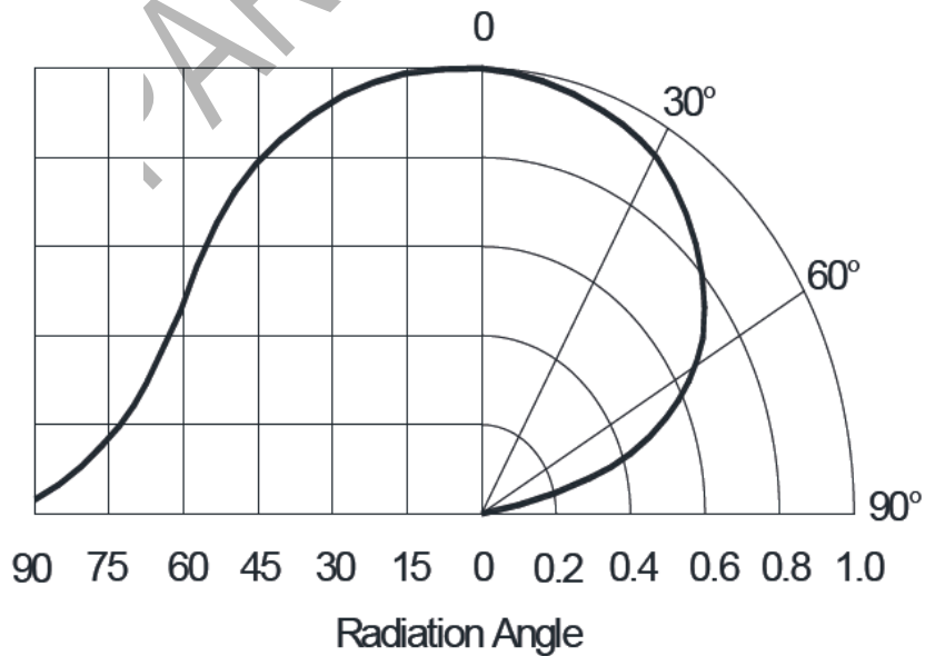
Typical Radiation Pattern 120°
