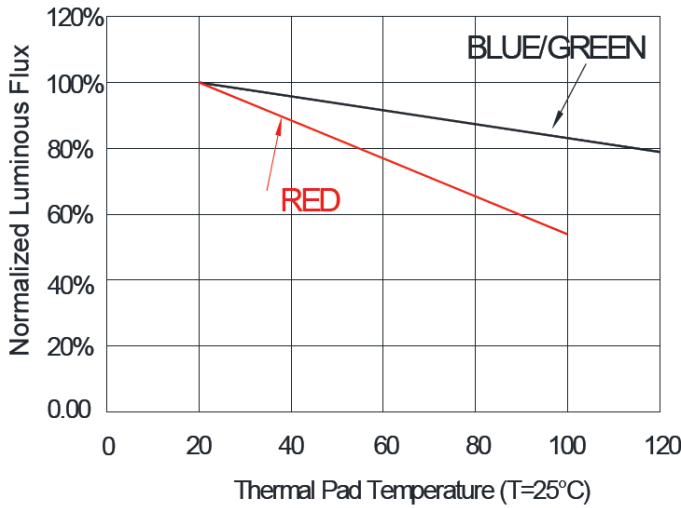
Thermal Pad Temperature vs. Relative Light Output
