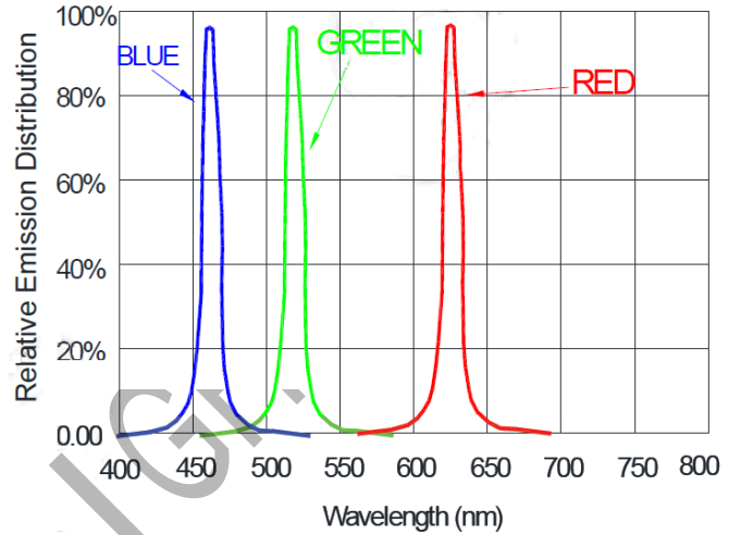
Wavelength Characteristics
