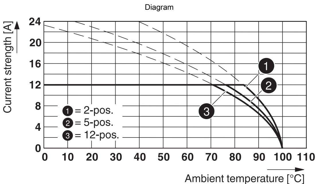
Type: FKVC 2,5/...-ST-5,08 with CCA 2,5/...-G-5,08 P26THR
