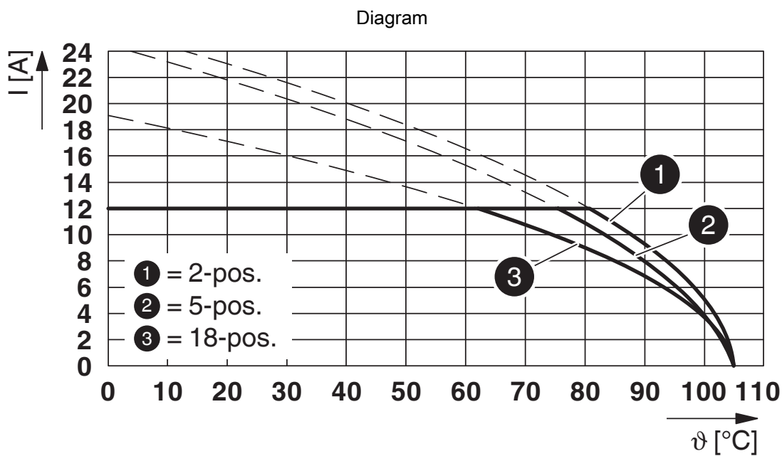
Type: FKCN 2,5/...-STF-5,08 with MSTB 2,5/...-GF-5,08
