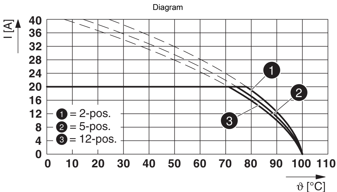
Type: PC 4/...-STF-7,62 with IPC 5/...-STGF-7,62
