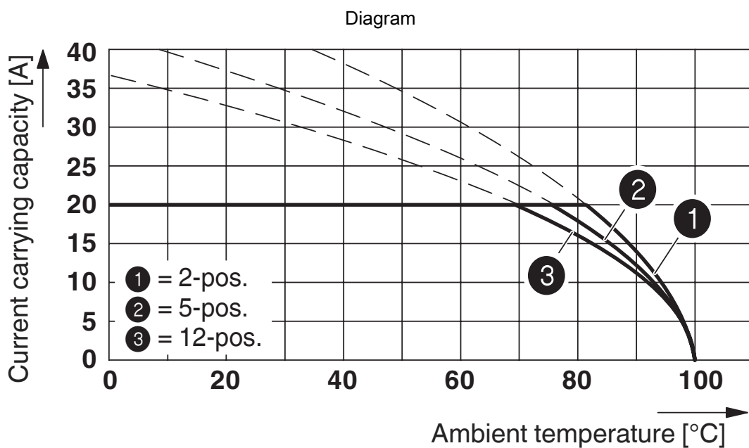
Type: PC 4/...-STF-7,62 with PC 4/...-G-7,62 and BF-PC 4
