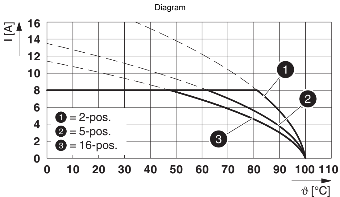
Type: FMC 1,5/...-STF-3,81 with MCD 1,5/...-GF-3,81
