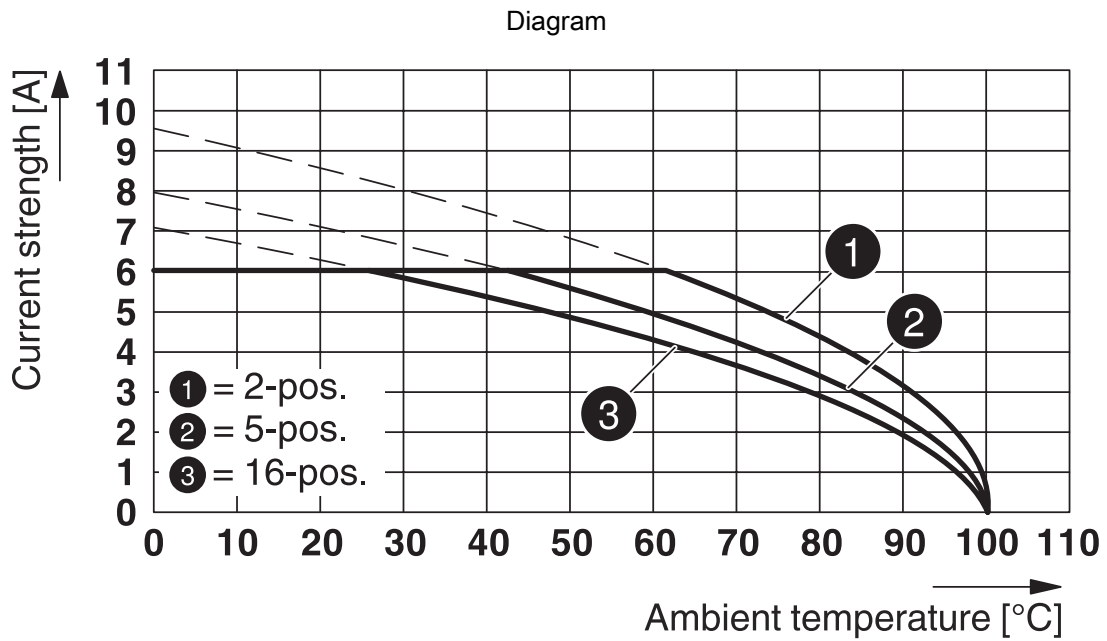
Type: DFMC 0,5/...-ST-2,54 with DMC 0,5/...-G1-2,54 P...THR R...
