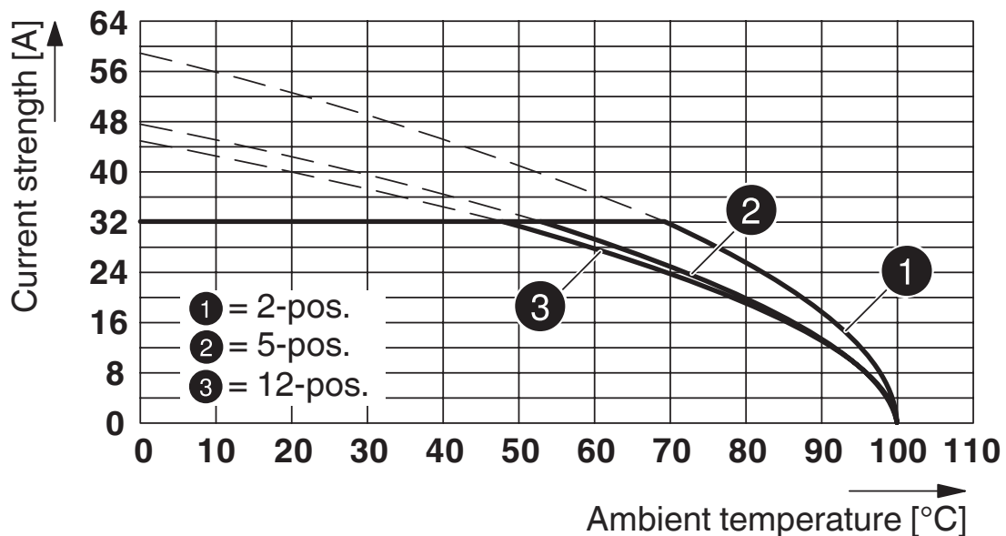
Type: TSPC 5/...-ST-7,62 with PC 5/...-G-7,62
